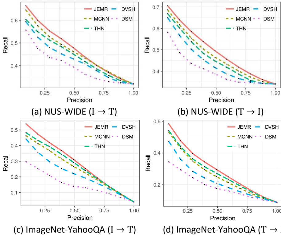
Figure 5: Precision-recall curves for the proposed method and the baselines for I \rightarrow T and T \rightarrow I tasks.
