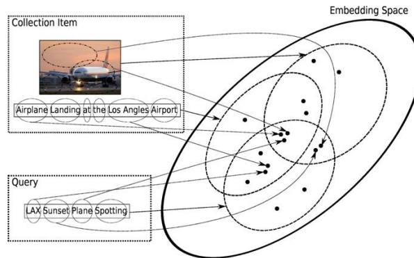
Figure 1: Projection of textual and visual components of an example query and multi-modal retrieval unit into the space of concept embeddings. The query term “plane” can be matched in both textual and visual components of a given retrieval unit, the query term “LAX” can be matched only in its textual component, while the term “sunset” can only be matched in its visual component.
