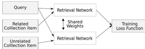
Figure 4: Procedure to train the parameters of the neural network in the last training stage.
