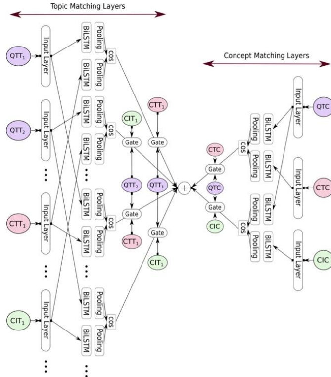
Figure 3: Projection layers in the proposed neural network architecture for T \rightarrow TI task. QTT_i , CTT_i and CIT_i are low-dimensional representations of the i -th topic in the query’s text, collection item’s text and collection item’s image, respectively. QTC , CTC and CIC are low-dimensional representations of concepts in query’s text, collection item’s text and collection item’s image.
