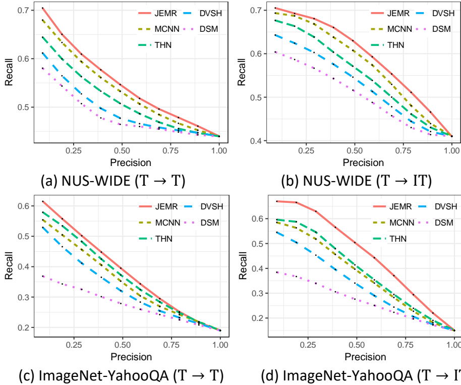
Figure 6: Precision-recall curves for the proposed method and the baselines for T \rightarrow T and T \rightarrow IT tasks.
