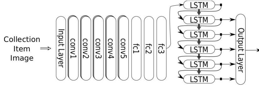
Figure 2: Image captioning layers in the proposed deep neural architecture for T \rightarrow T task. A combination of convolutional layers conv1-conv5 and fully connected layers fc1-fc3 is used for image feature extraction. LSTM is used for caption generation.
